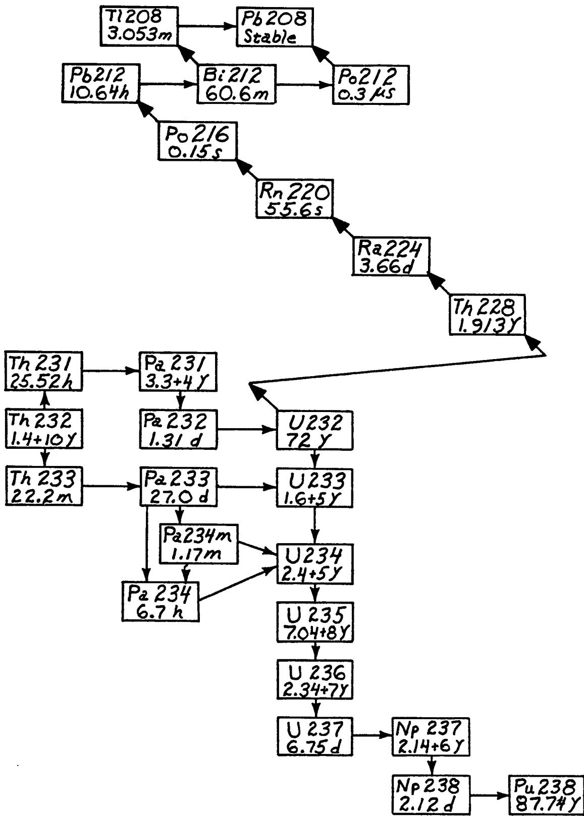
Fig. E-13. Actinide nuclides important to decay power in U 233 /Th 232 -fueled light water reactors.
