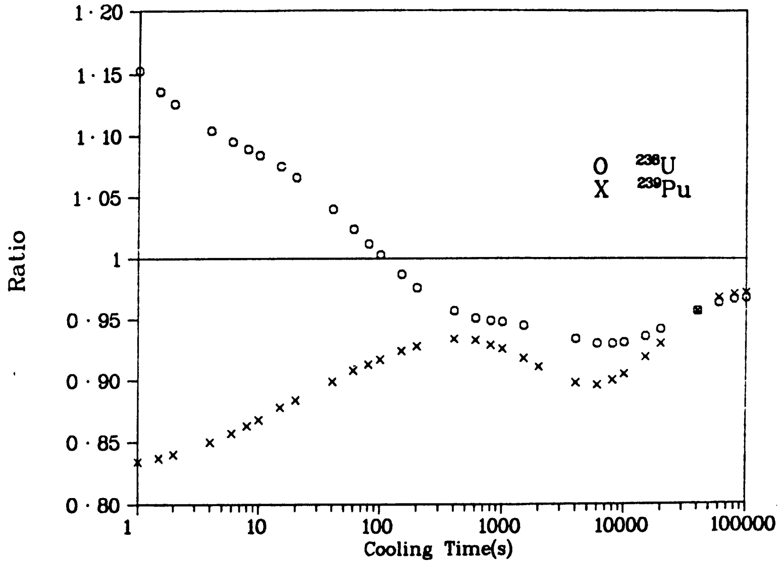
Fig. A-3. Ratio of ^{239}\text{Pu} and ^{238}\text{U} nominal decay heating to ^{235}\text{U} nominal - infinite irradiation.
